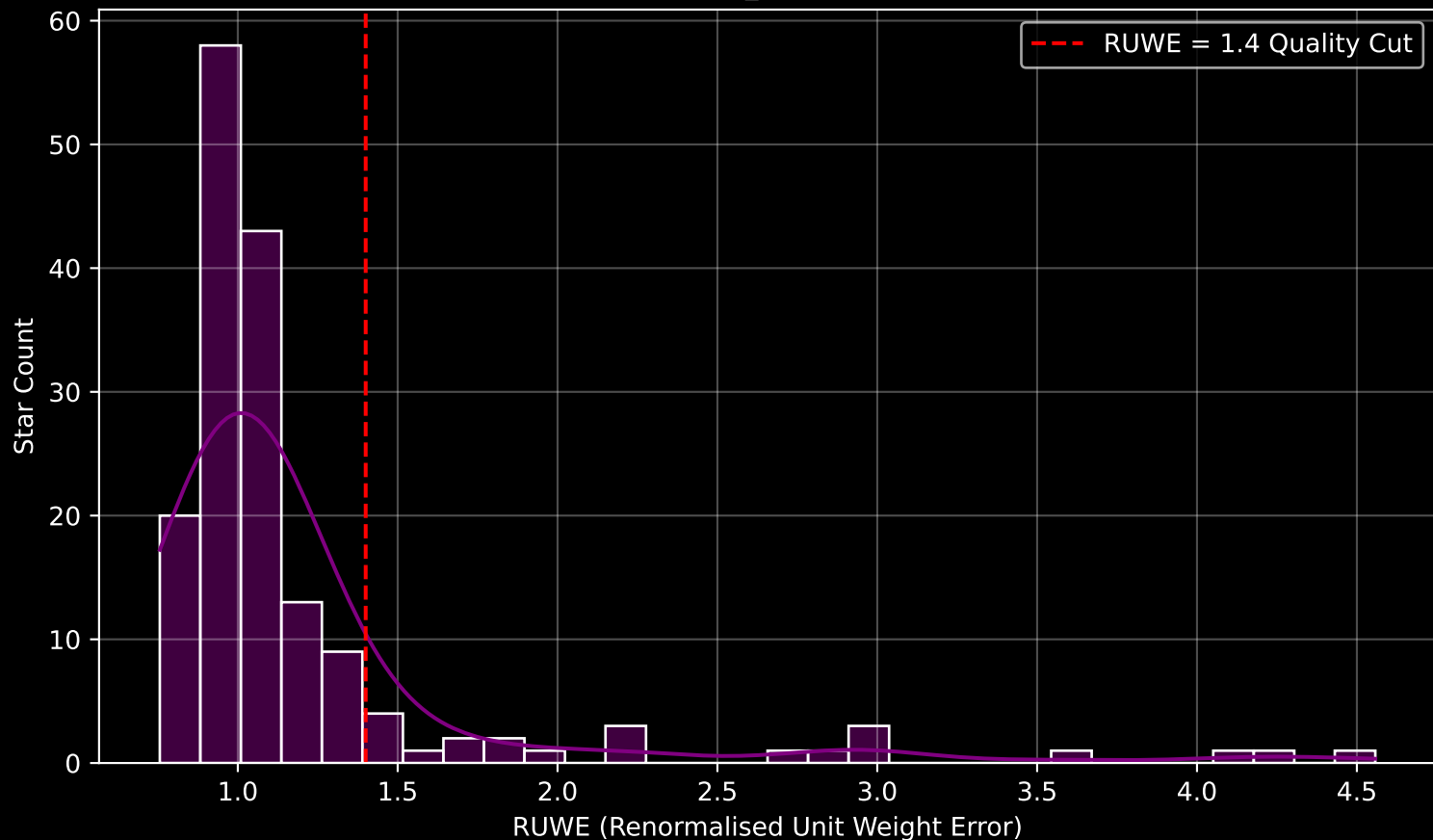
GAPOGEE DR17 Field [273-26-O_TESS] RUWE Distribution (n= 165)
